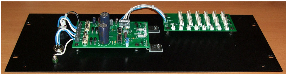
A standard 4U high 19" panel with an issue 2 Oakley PSU and single Dizzy. This would be suitable for powering up to 12 Oakley modules. Note the grounding point just below the main power inlet.
