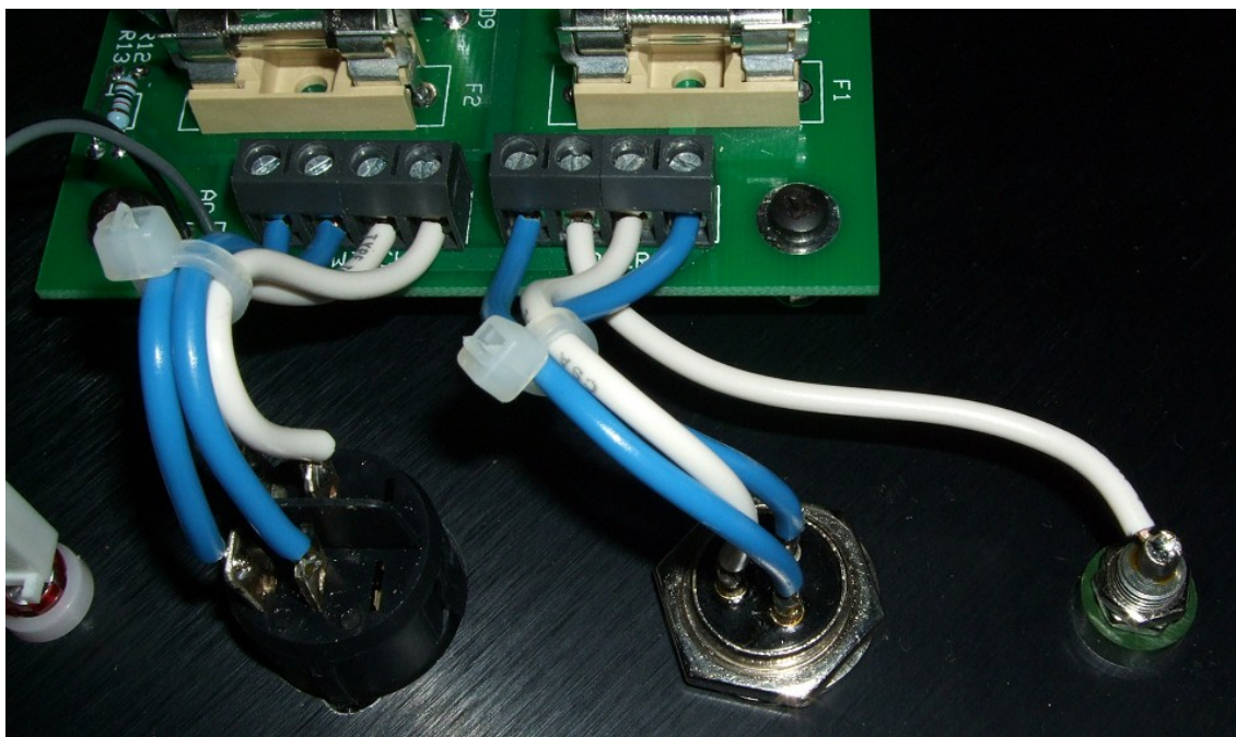
A 4mm banana socket being used as a common grounding point for a rack power supply. Here the banana socket is connected directly with a nice thick piece of wire to the spare 0V1 screw terminal.
