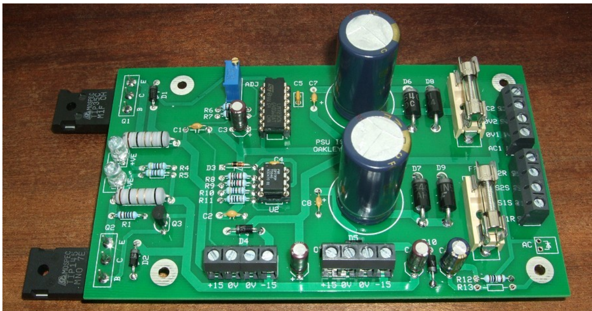
The issue 2 Oakley PSU board awaiting fitting to the front panel.
