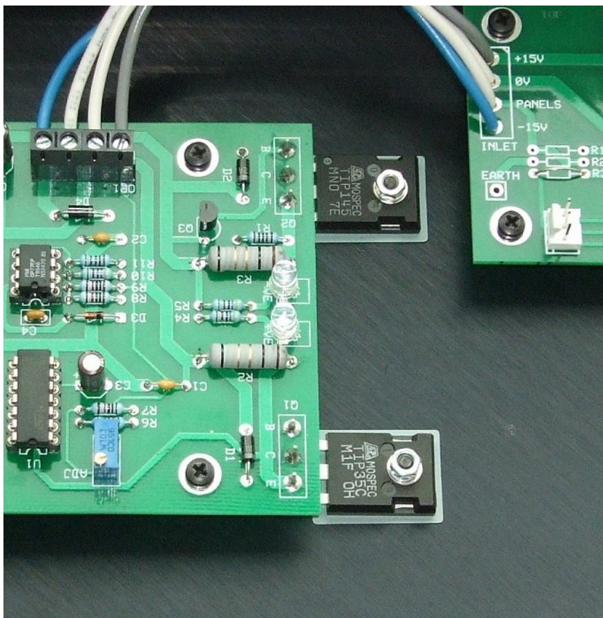
The MOSPEC devices mounted onto their panel – in this case it's the 19" 4U high rack panel. You can see the grey insulating sheets between the power devices and the panel.
