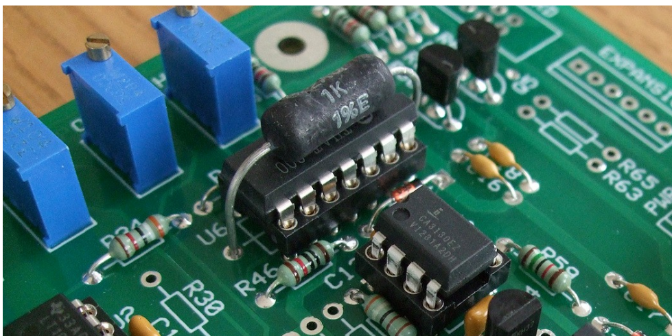
A close up of the VCO core. Note the positioning of the positive temperature coefficient (PTC) resistor. The PTC straddles U6 and a small amount of thermal paste can be used to keep them both at the same temperature.
