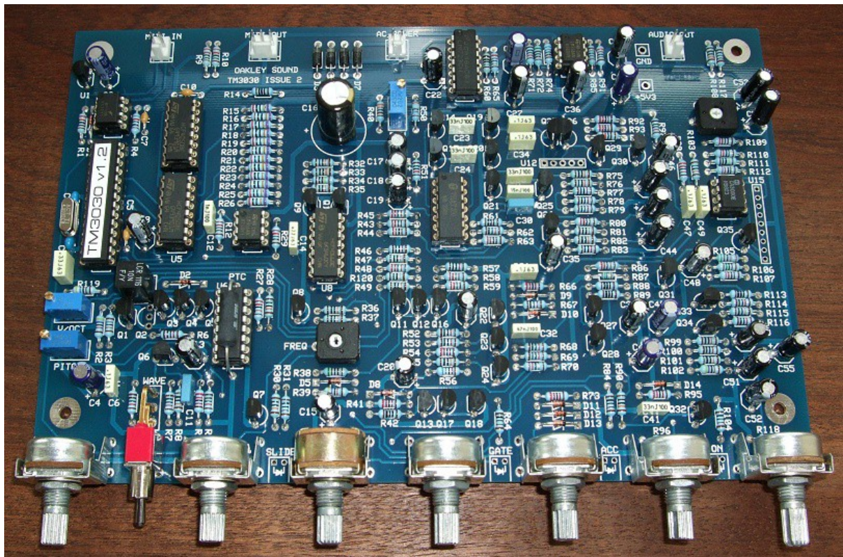
An issue 2 board awaiting its case and LEDs. This one has been built with a matched BC550B pair in the VCF and a CA3080 and discrete buffer for the VCA.
