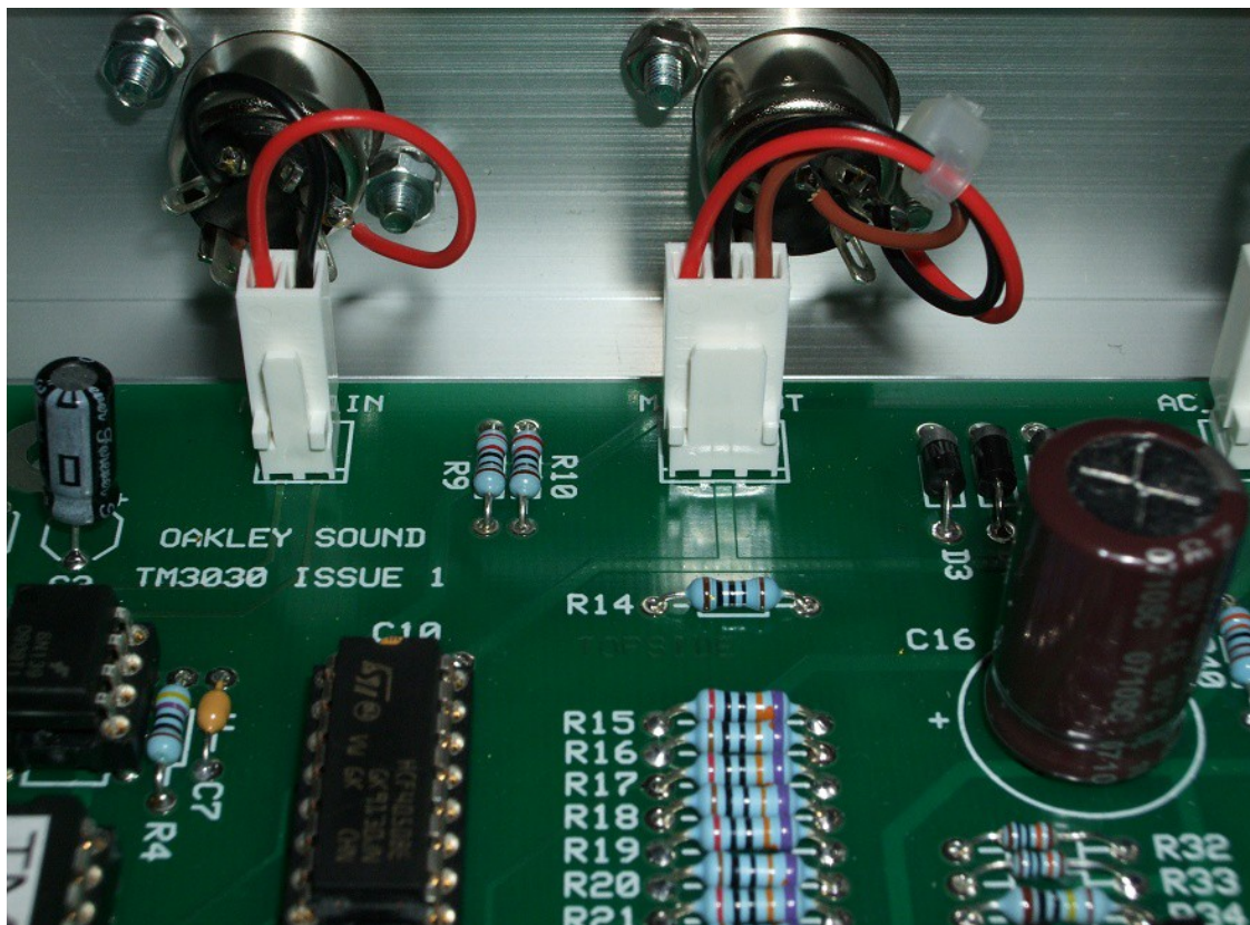
A close up of an older issue 1 TM3030 showing the midi connections done with Molex KK 0.1" headers and housings. Issue 2 boards can be wired in a similar way.
