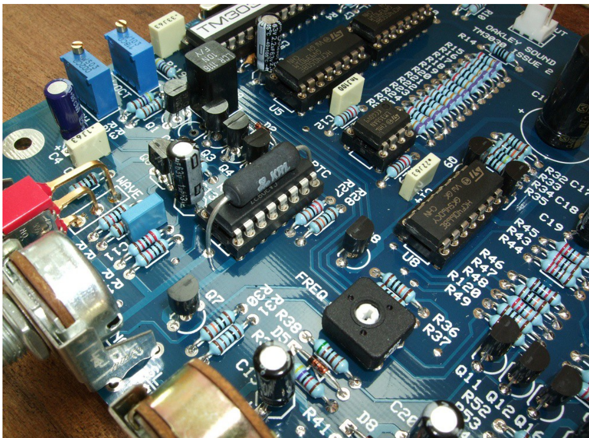
A close up of the VCO circuitry of the TM3030. Note the positioning of the positive temperature coefficient (PTC) resistor. Although not used here, a small amount of thermal paste can be used to keep both U6 and the PTC at the same temperature.
